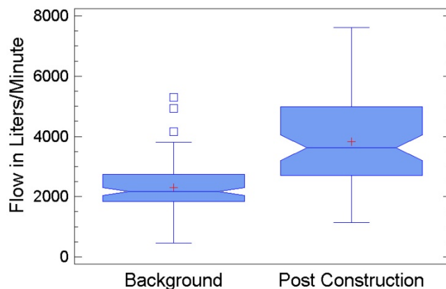
Figure 2. Notched box-and-whisker plot illustrating the flow rate differences observed before and after construction of the treatment plant.
