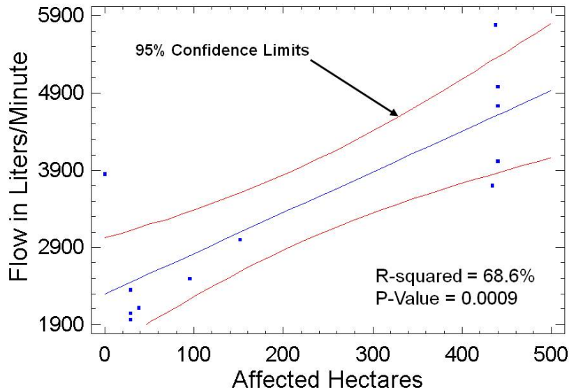
Figure 3. Regression analysis illustrating the relationship of mean annual discharge rate to amount of drainage area affected by surface mining.
