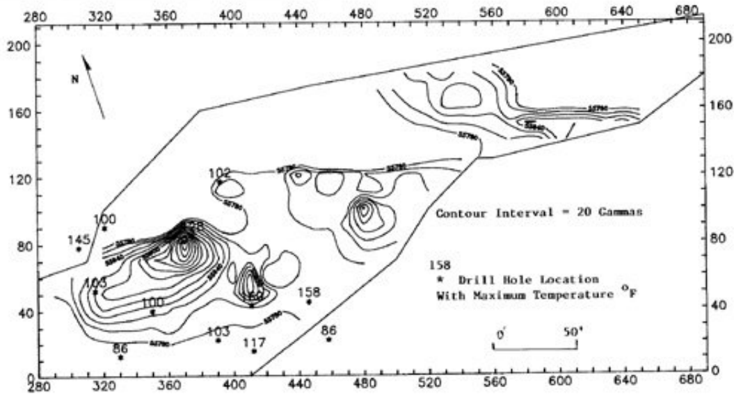
FIGURE 3. POSITIVE MAGNETIC ANOMALIES RECORDED AT SWRB1.
