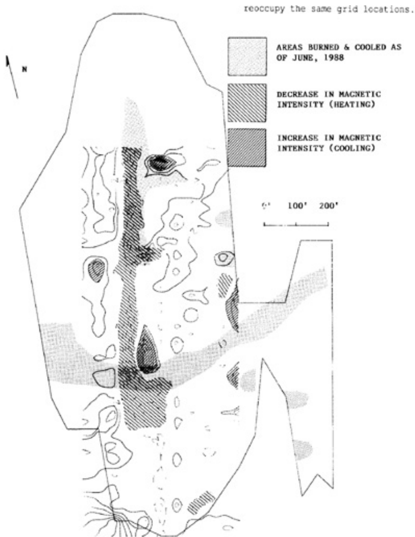
FIGURE 2. DMFI CHANGES IN MAGNETIC INTENSITY BETWEEN JUNE, 1988 & JUNE, 1989
