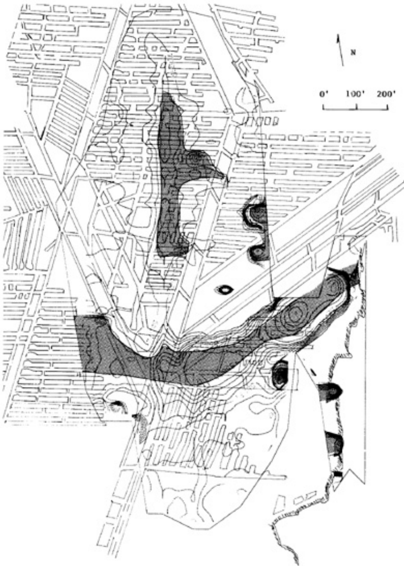
FIGURE 1. DMFI POSITIVE MAGNETIC ANOMALIES SUPERIMPOSED OVER DEEP MINE WORKINGS. SHADED AREAS SHOW AREAS INTERPRETED TO HAVE BURNED AND COOLED.
