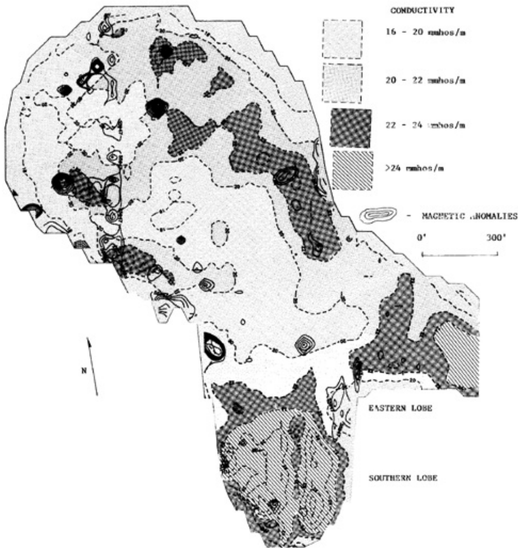
FIGURE 4. POSITIVE MAGNETIC ANOMALIES AT NCPAI SUPERIMPOSED ON EM CONTOUR PLOT
