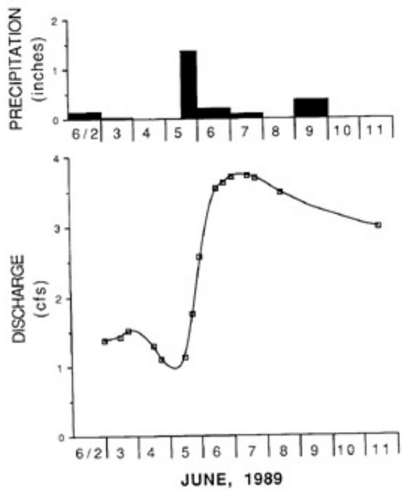
Figure 10. Precipitation and discharge hydrograph for Spring #1 (June 2–11, 1989).
