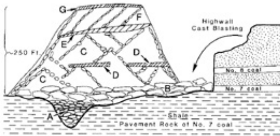
Figure 4. Schematic cross section showing components of spoil significant to the development of an aquifer framework: A = hollow fill, B = cast-blasted rubble, C = dragline spoil, D = dragline pad, E = temporary haul road, F = end-dumped spoil, and G = final graded land surface.
