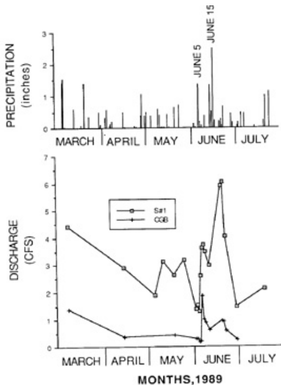
Figure 11. Precipitation and discharge hydrograph for Spring #1 and Chestnut Gap Branch (March 1–July 25, 1989).
