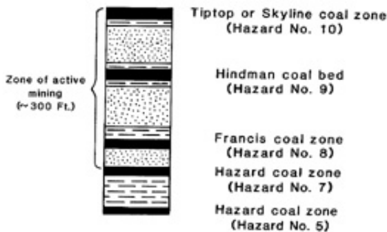
Figure 2. Schematic geologic column of site.
