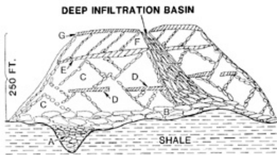
Figure 6. Schematic cross section showing components of spoil significant to the development of an aquifer framework: A = hollow fill, B = cast-blasted rubble, C = dragline spoil, D = dragline pad, E = temporary haul road, F = end-dumped spoil, and G = final graded land surface.
