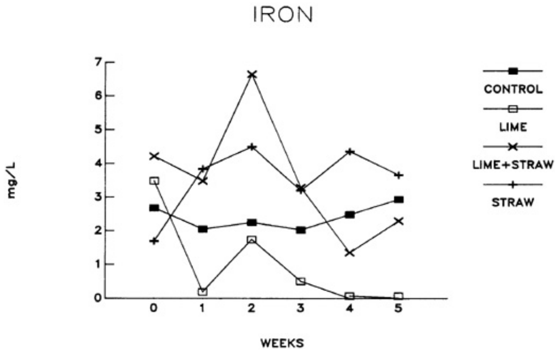
Figure 6: Iron concentrations at the 3 m level in the experimental enclosures.
